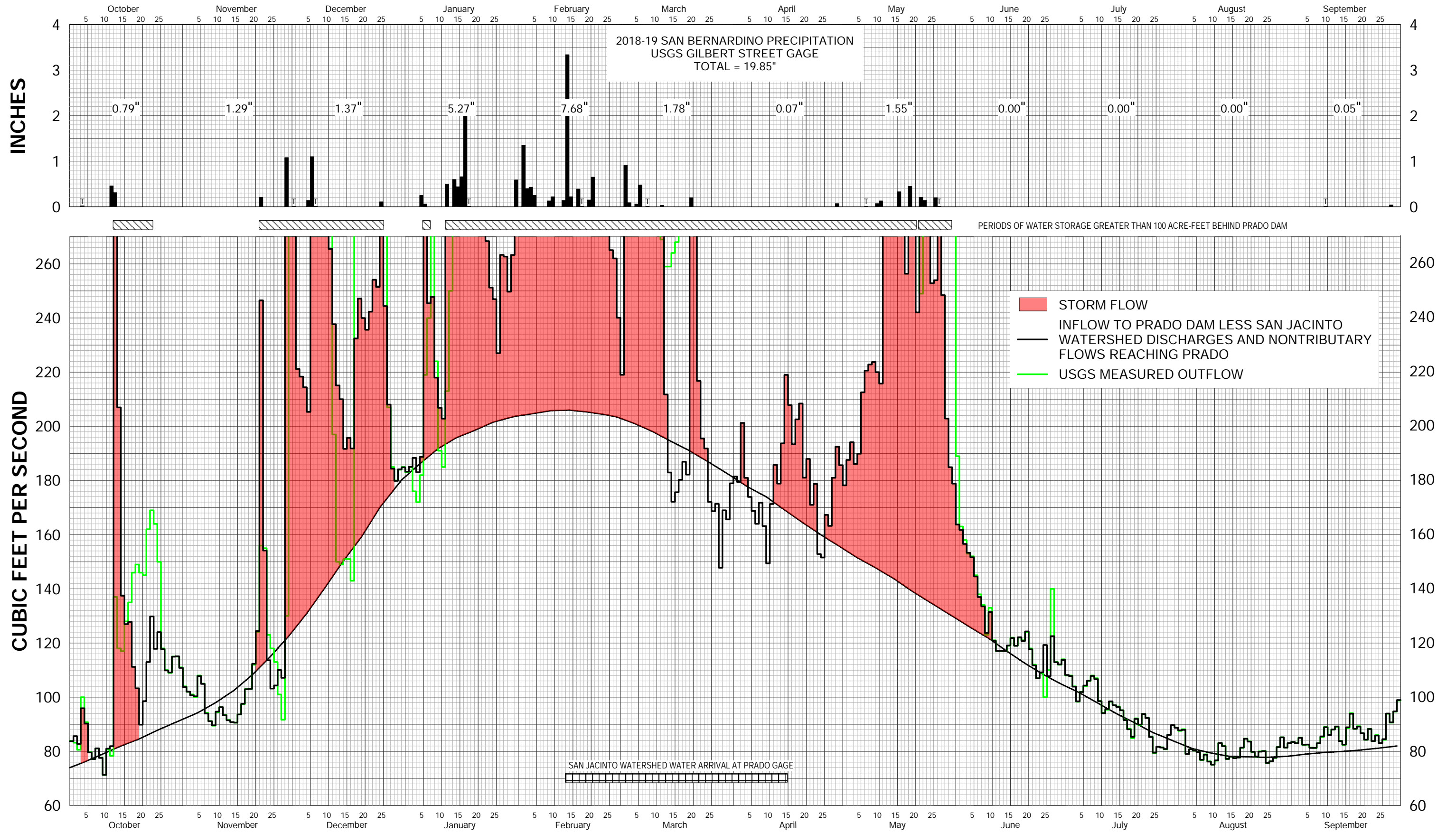
DISCHARGE OF THE SANTA ANA RIVER AT PRADO DAM & SAN BERNARDINO PRECIPITATION WATER YEAR 2018-19
