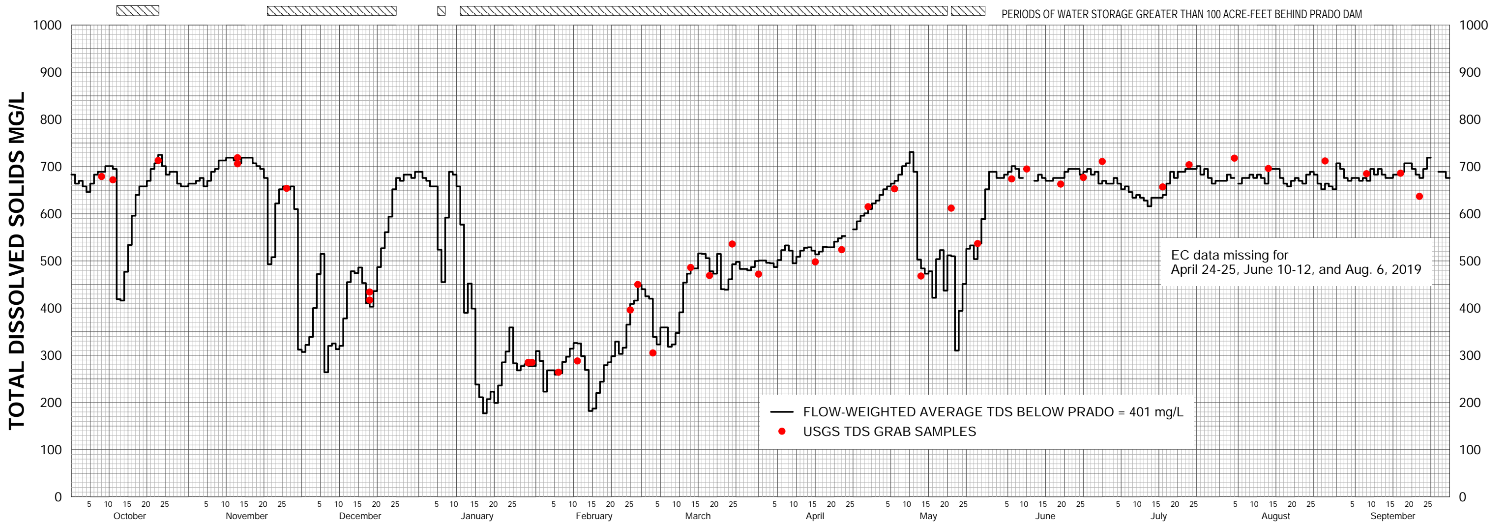
DISSOLVED SOLIDS IN SANTA ANA RIVER BELOW PRADO DAM WATER YEAR 2018-19
