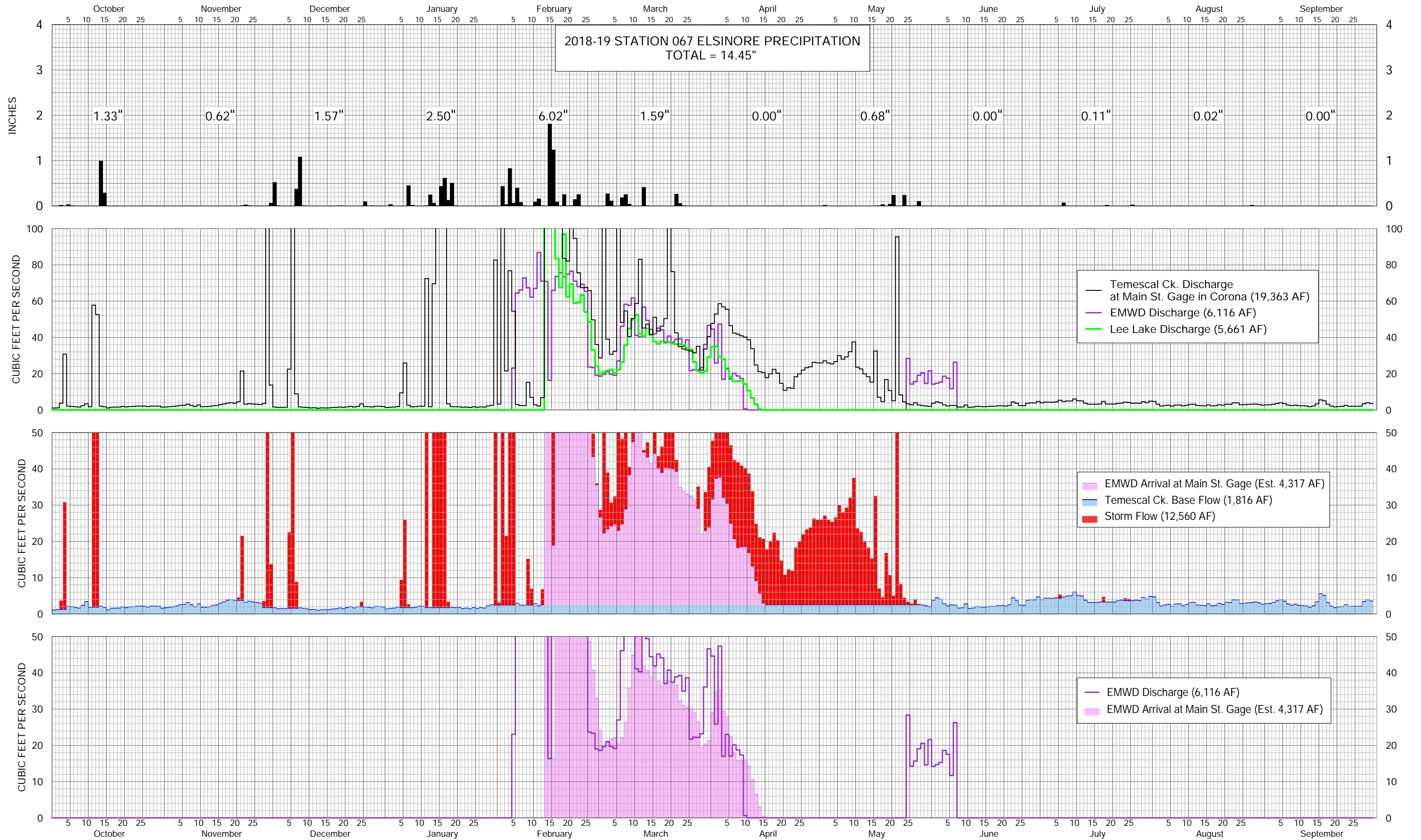
WATER YEAR 2018-19 PROVISIONAL DISCHARGE OF TEMESCAL CREEK AT MAIN STREET IN CORONA, LEE LAKE DISCHARGE, EMWD DISCHARGE, AND ELSINORE PRECIPITATION
