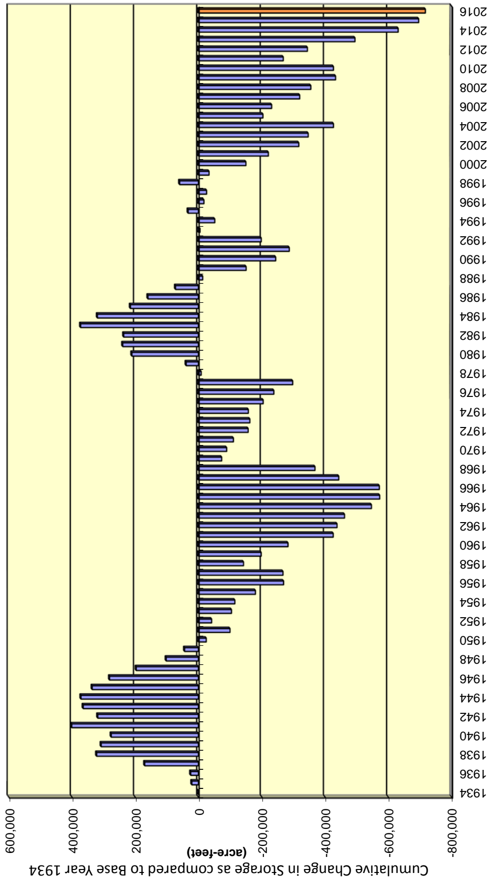
Cumulative Change in Storage for the San Bernardino Basin Area
