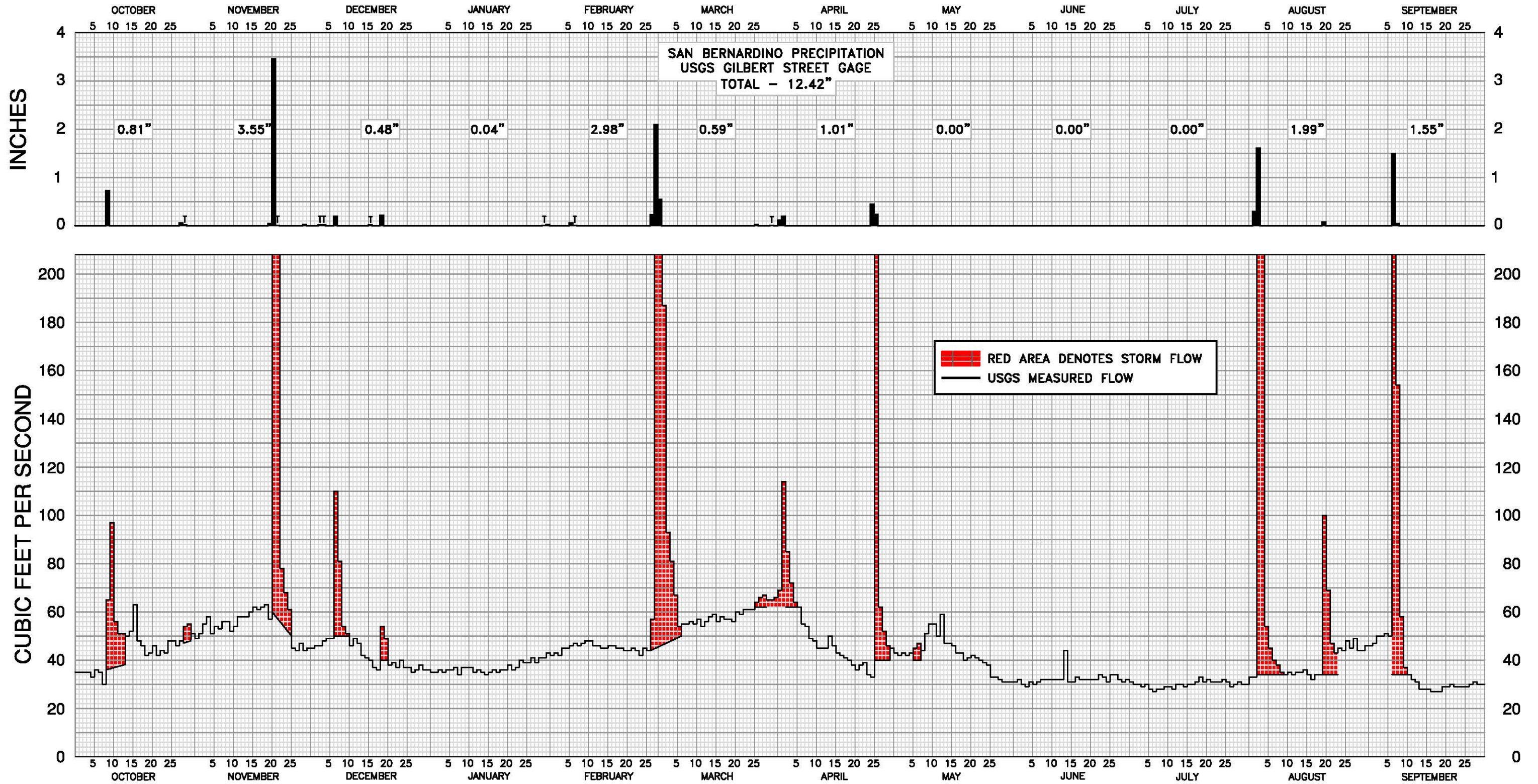
DISCHARGE OF SANTA ANA RIVER AT RIVERSIDE NARROWS & SAN BERNARDINO PRECIPITATION WATER YEAR 2013-14
