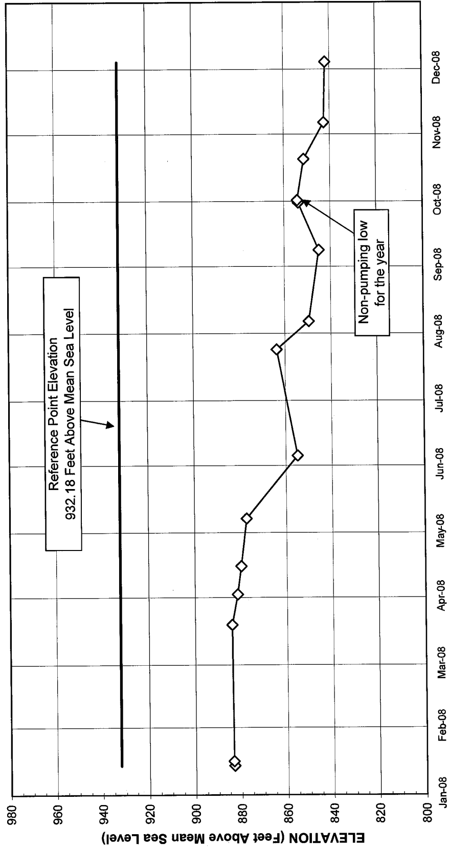
FIGURE 2 GROUNDWATER SURFACE ELEVATIONS 1S/4W-29H01S FLUME NO. 2 WELL 2008
