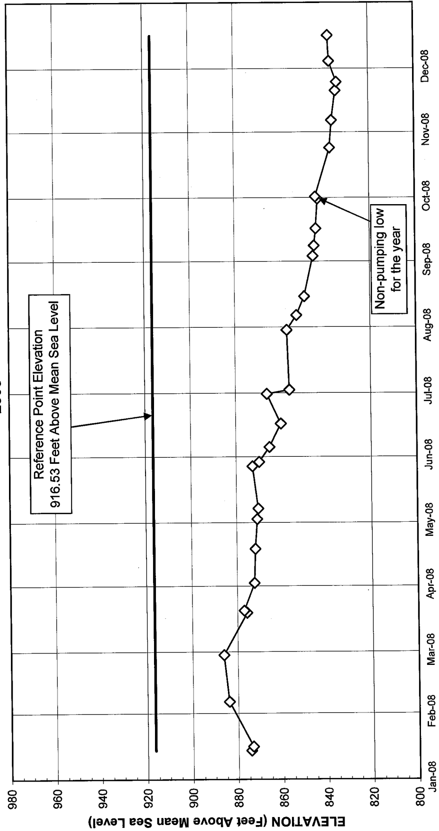
FIGURE 3 GROUNDWATER SURFACE ELEVATIONS 1S/4W-29Q01S FLUME NO. 5 WELL 2008
