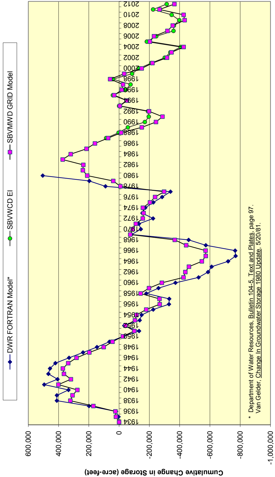
Figure 2. Comparison of DWR FORTRAN Model, SBWCD EI and SBVMWD GRID Model Results
