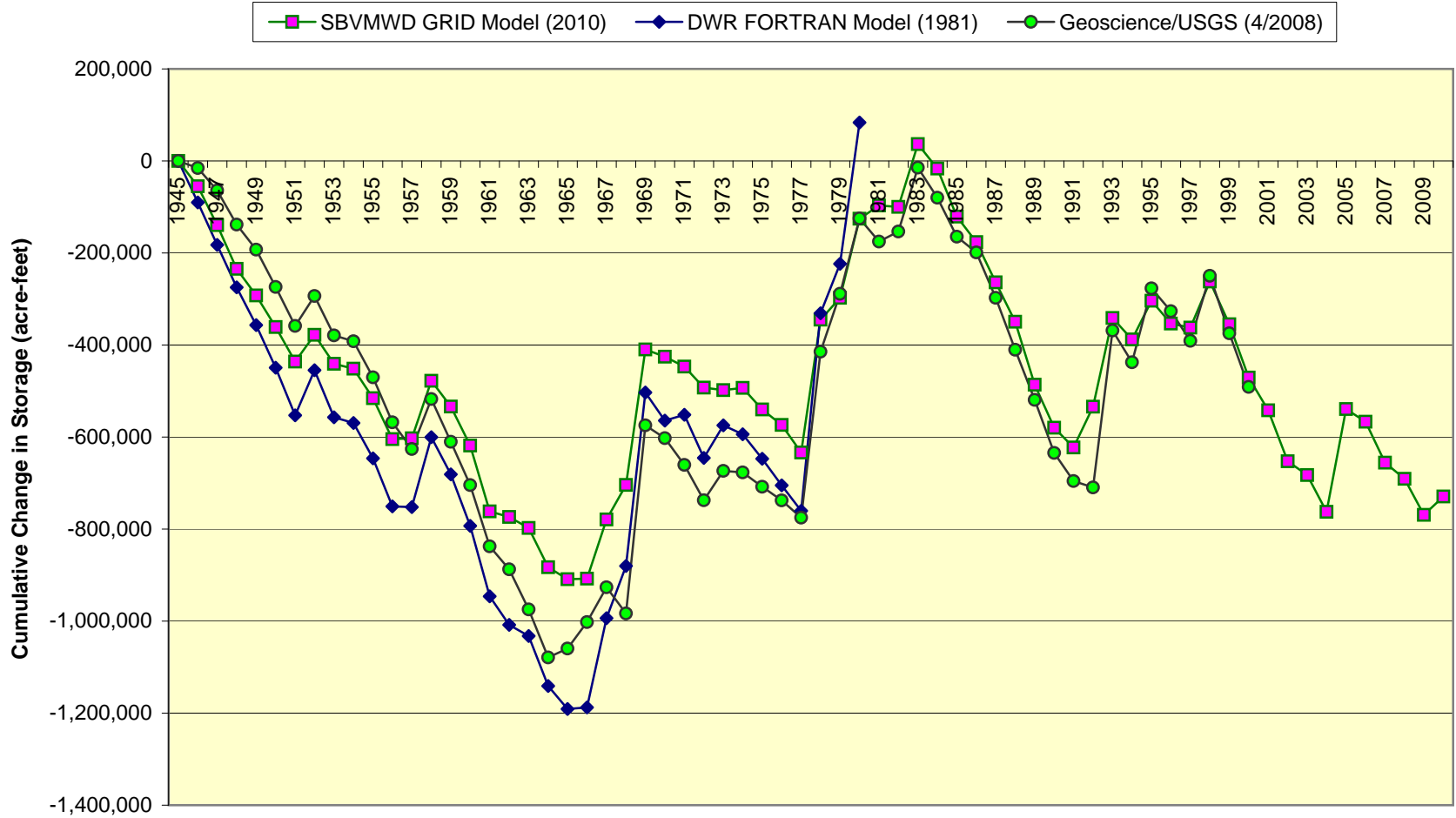
Figure 1.2. Comparison of DWR FORTRAN Model, USGS MODFLOW Model and SBVMWD GRID Model Results
