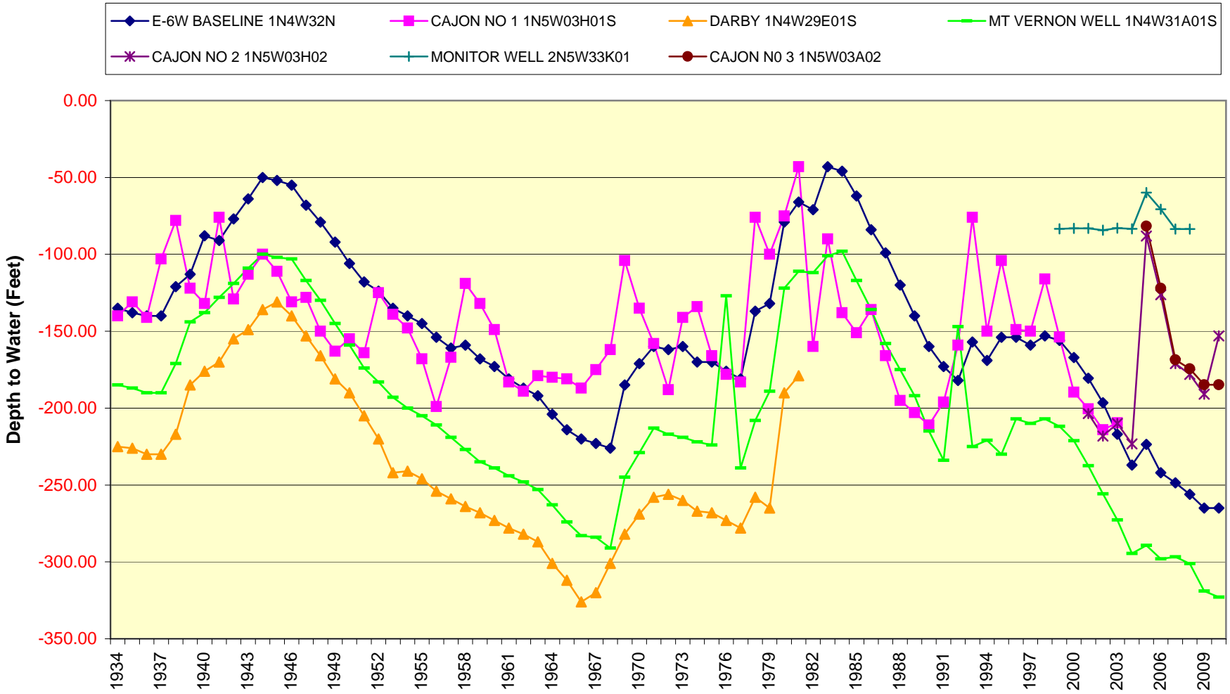
Hydrographs for the Cajon Sub-Basin Wells
