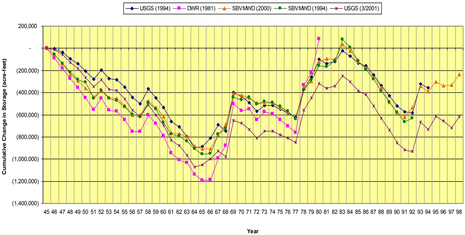
Figure B.1.1. Comparison of DWR FORTRAN Model, USGS MODFLOW Model and SBVMWD GRID Model Results
